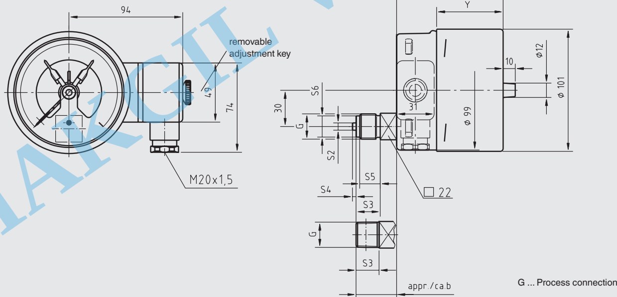
Lower back mount
