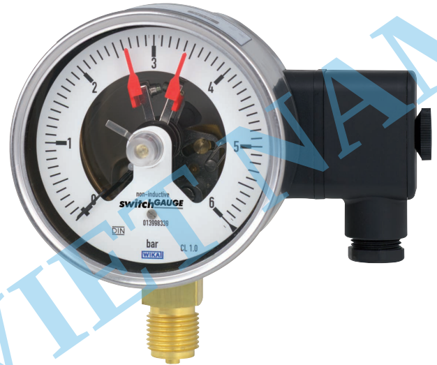
Model PGS21.100 with model 821.21 switch contacts
